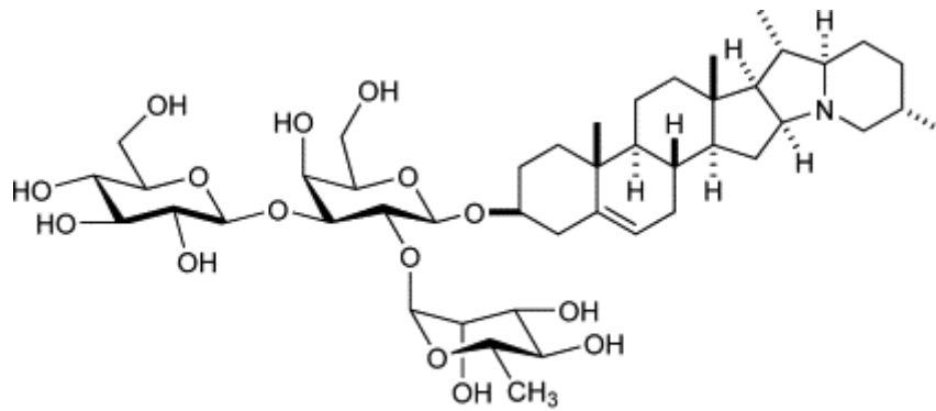
Solanine
